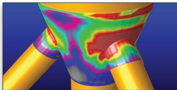
Parametric study for the fatigue design of a wind turbine transition piece.
