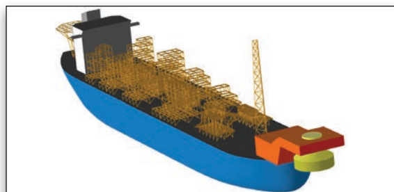
Data interchange with MOSES for FPSO topsides analysis.
